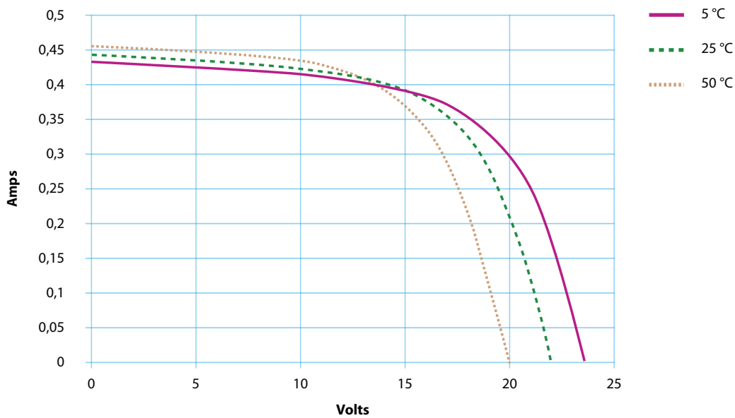
I-V curves as a function of temperature, irradiation = 1000W/m²
