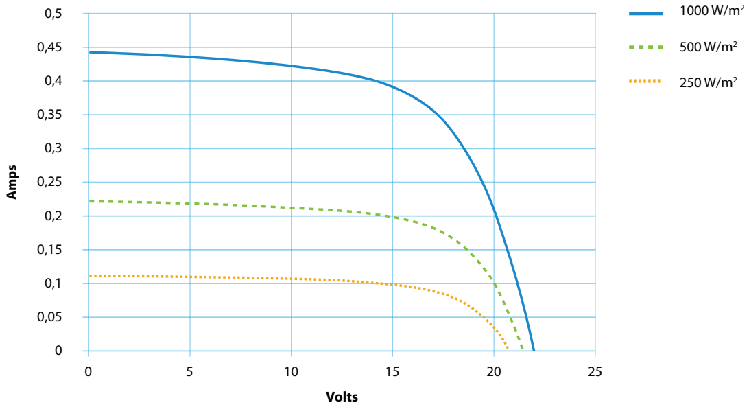
I-V curves as a function of irradiation, temperature = 25 °C
