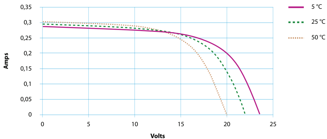
I-V curves as a function of temperature, irradiation = 1000W/m 2
