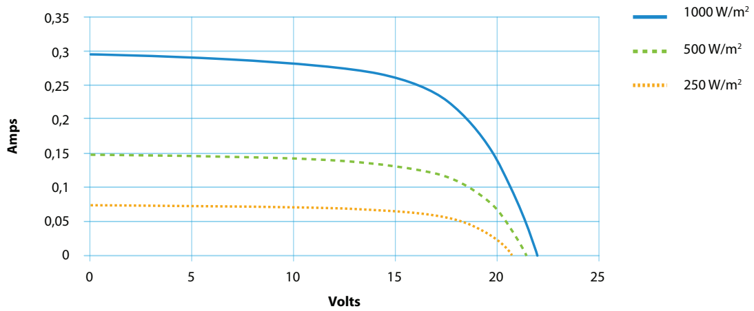
I-V curves as a function of irradiation, temperature = 25 °C
